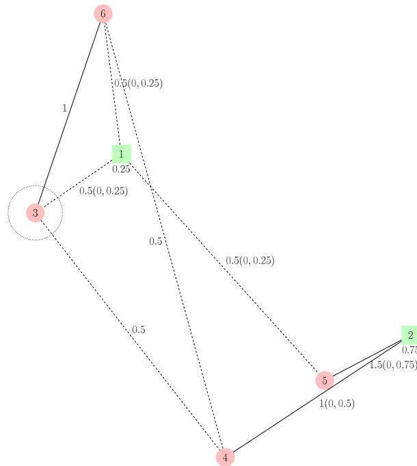
Fig. 1. Fractional solution of (VF2) violating y -GLM by 0.19 with z = 561.3 .
