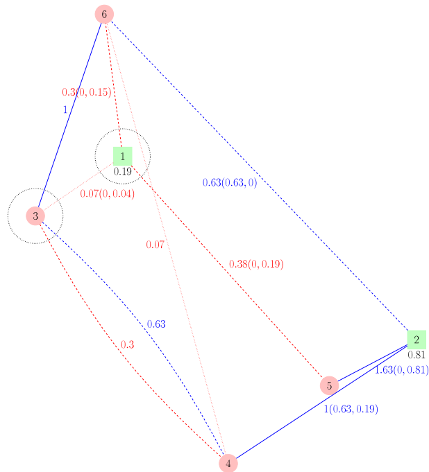
Fig. 3. Fractional solution of (VF3) violating y -LRGLM by 0.14 with z = 587 .
