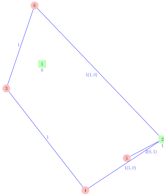
Fig. 4. Fractional solution of (CF3) with z = 594 .
