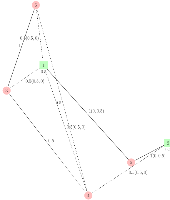
Fig. 2. Fractional solution of (CF2) with z = 593.5 .
